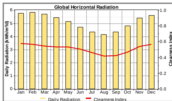
Figure 2: Solar Radiation and Clearness Index of the Study Area (NASA)
