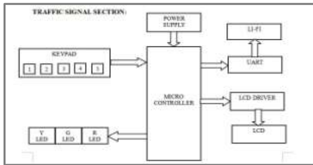
Figure 1: Block Diagram of Traffic Signal Section
