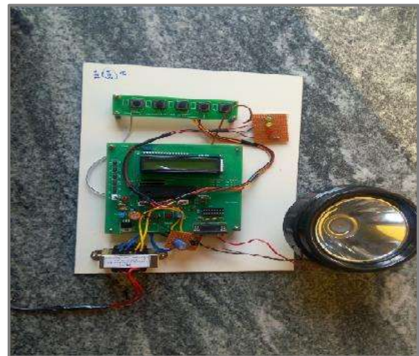
Figure 4: Transmitter
