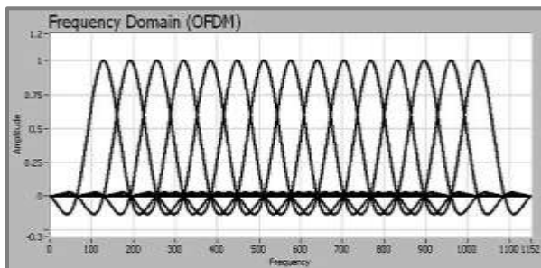
Figure 3: OFDM Signal Generation
