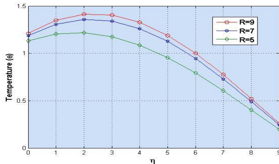
Figure 7: Temperature Graph against Plate Distance when Varying Radiation Parameter
