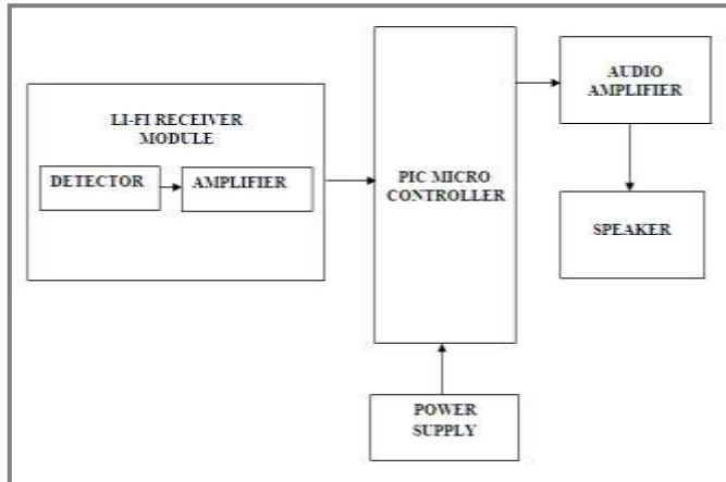
Figure 3: Li-Fi Receiver
