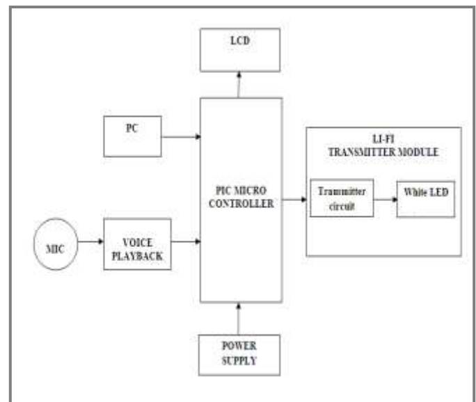
Figure 1: Li-Fi Transmitter
