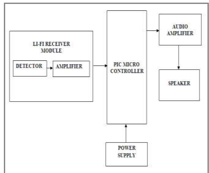
Figure 2: Receiver
