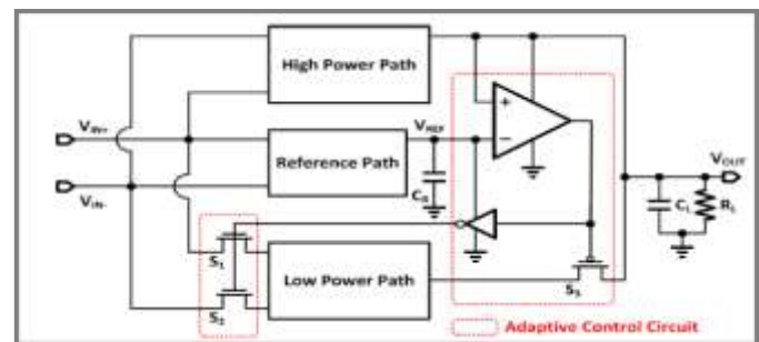
Figure 2: System Architecture of the Dual-Path Rectifier
