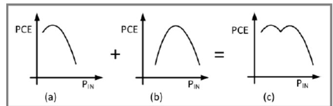
Figure 1: Efficiencies of the Conventional Rectifier (a) Optimized at Low Power, (b) Optimized at High Power, and (c) The PCE of the Proposed Dual-Path Rectifier
