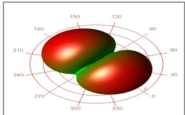
Figure 6: Radiation Pattern of Microstrip Patch Antennas with SRR Structure at 5.8GHz
