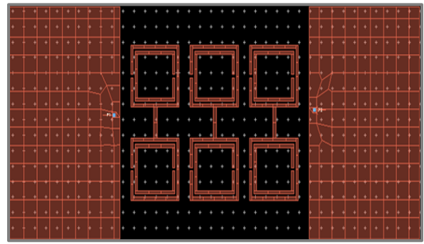
Figure 1: Geometry of Microstrip Patch Antennas with SRR
