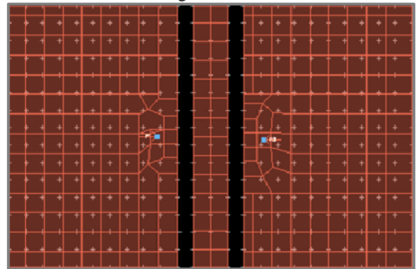
Figure 2: Proposed Microstrip Patch Antennas with WG-MTM
