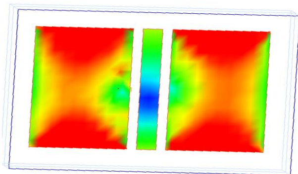
Figure 5: Simulated Electric Current Distribution of the Microstrip Patch Antennas with WG-MTM at 5.8GHz
