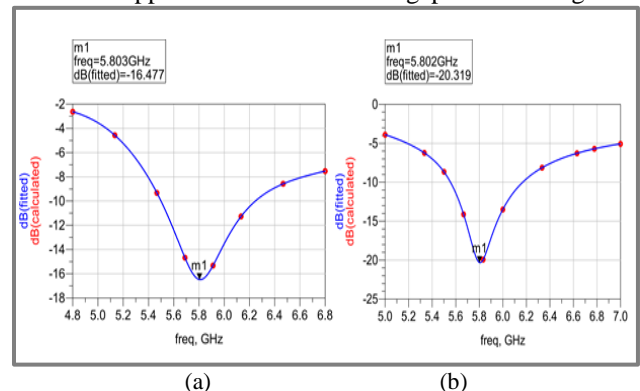
Figure 3: S Parameter Plots for Return Loss Vs. Frequency for Microstrip Patch Antennas with Isolation: (a) SRR, (b) WG-MTM
