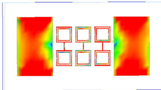
Figure 4: Simulated Electric Current Distribution of the Microstrip Patch Antennas with SRR at 5.8GHz
