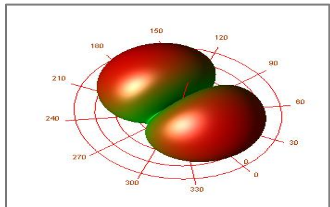
Figure 7: Radiation Pattern of Microstrip Patch Antennas with WG-MTM Structure at 5.8GHz
