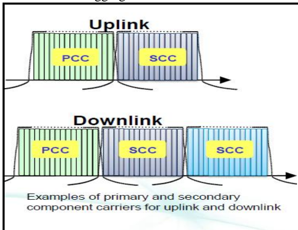
Figure 3 – Symmetric and Asymmetric Carrier Aggregation
